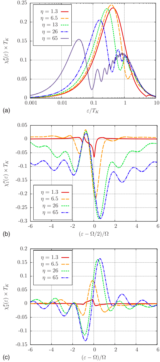
FIG. 5. (Color online) Universal curves of the zeroth, first, and second mode \chi_n''(\epsilon - n\Omega/2) for different values of the parameter \eta .
