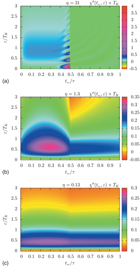
FIG. 4. (Color) False color plots of the dynamical susceptibility \chi''(t_{\text{av}}, \varepsilon) at a given point t_{\text{av}} in time for different values of the parameter \eta . The upper plot shows the behavior for slow driving consistent with a single interaction quench picture. The lower plot displays the fast-driving behavior that is similar to an equilibrium problem. The plot in the middle shows the intermediate regime of competing time scales.
